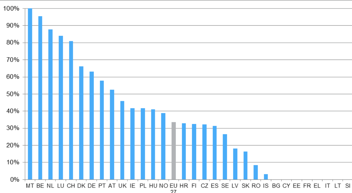
DOCSIS 3.1 by country, 2023
