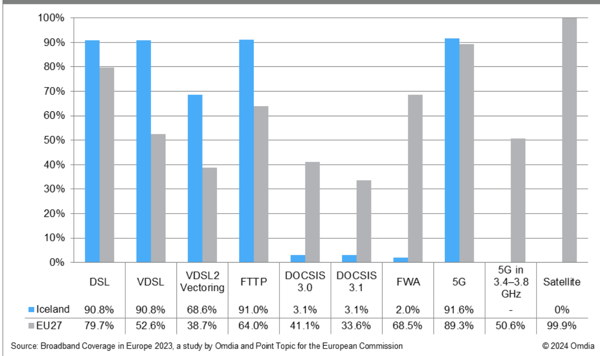
Iceland: Coverage by technology, total, 2023
